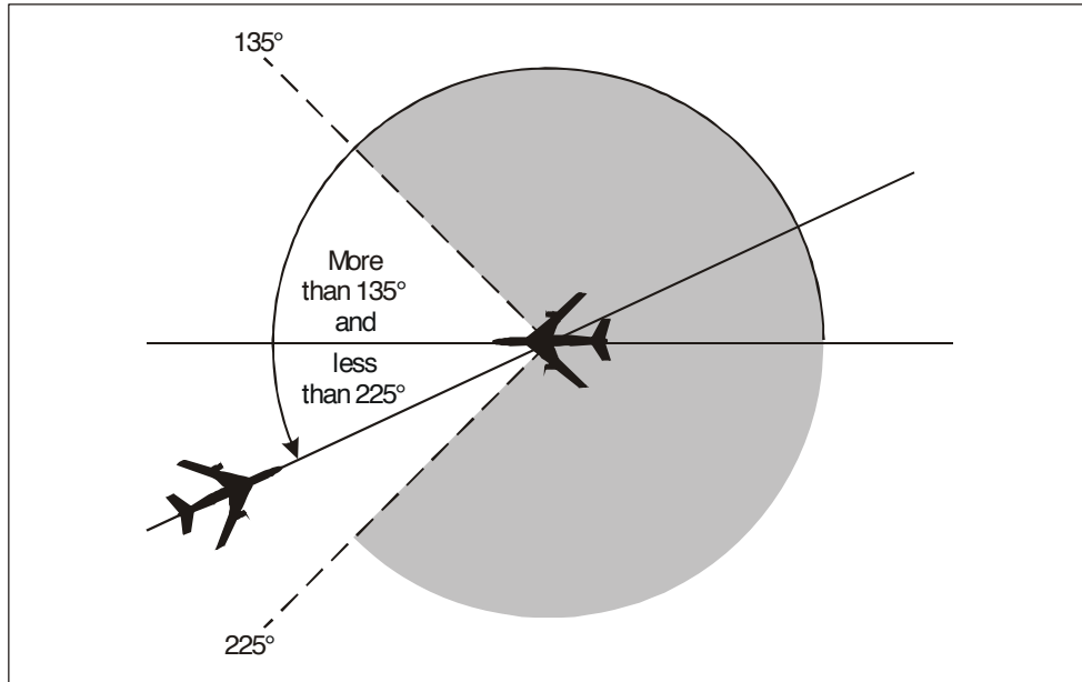
Figure 5-8. Aircraft on reciprocal tracks (see 5.4.2.1.5 b))
